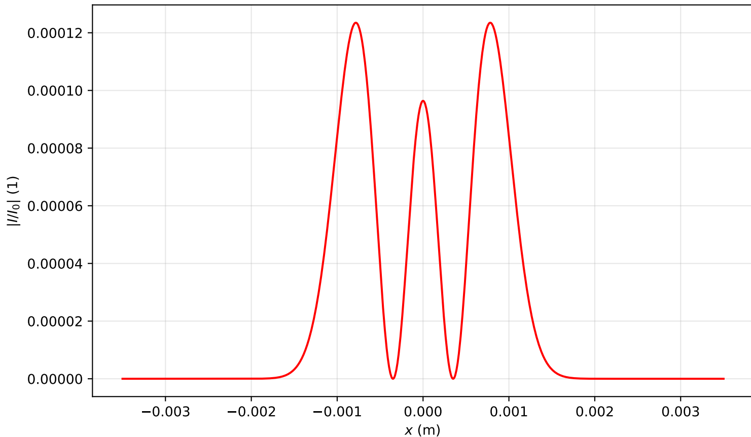
Intensity profile I(x, y = 0, z = 0.080)/I_0 , P_{in}=8.0P_{cr} , artificial time
